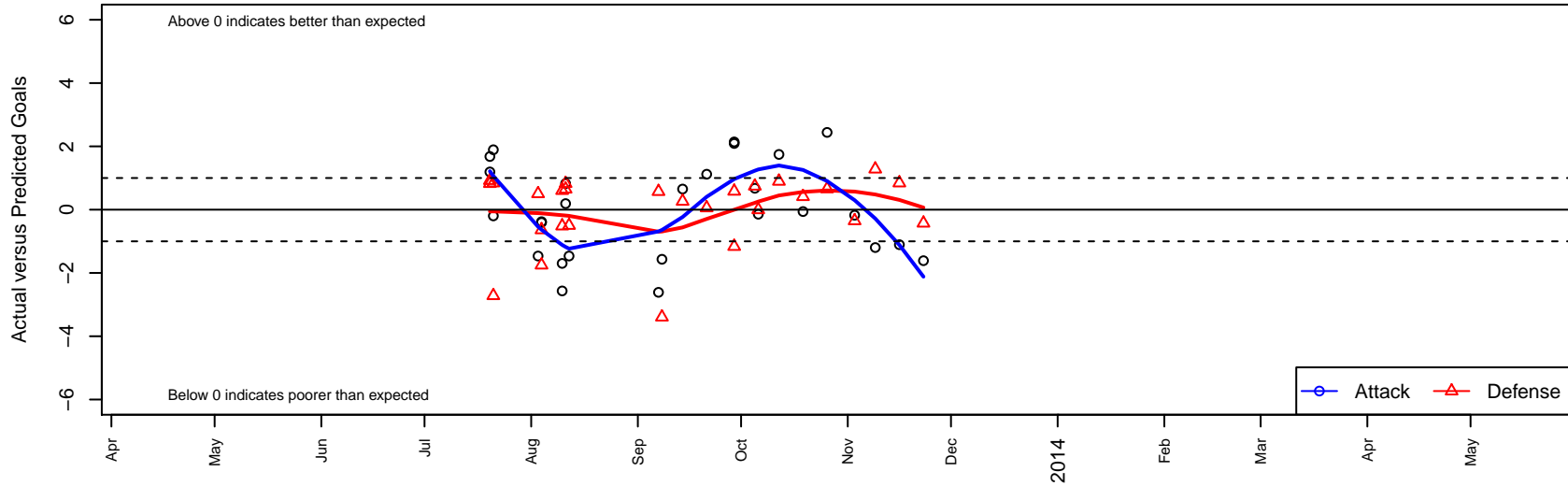
Strikers FC Irvine B02 Dots are actual minus expected GF (blue circles) and GA (red triangles). Blue line is smoothed change in attack strength. Red is smoothed change in defense strength.
